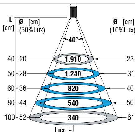
MN03 L40-F700-24ACDC
