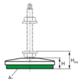
Dimensioned sketch
